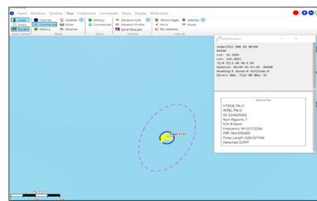
Zoomed in display of the 'hooked' radar return with data and associated location error ellipse.
